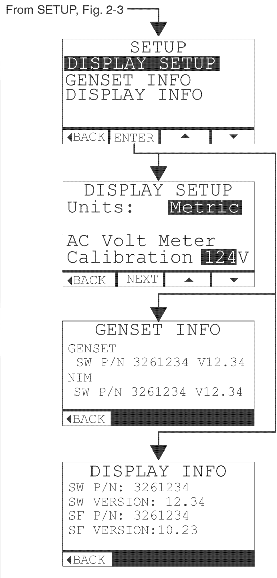
FIGURE 8. TYPICAL SETUP SCREENS
